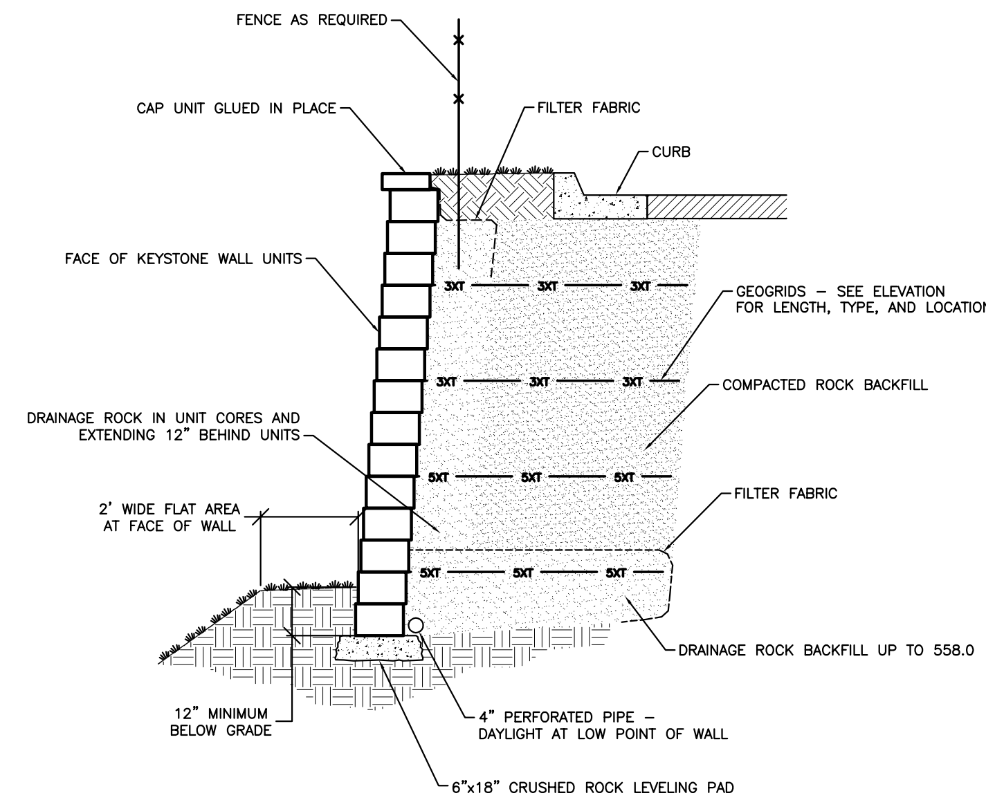
TYPICAL SECTION NOT TO SCALE
