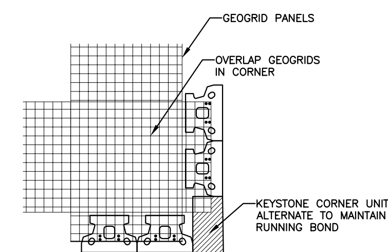
OUTSIDE CORNER DETAIL NOT TO SCALE
