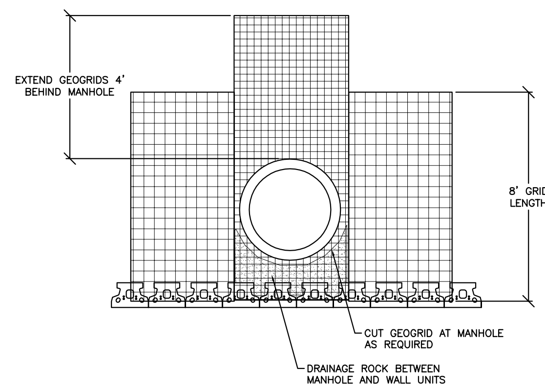
MANHOLE DETAIL NOT TO SCALE
