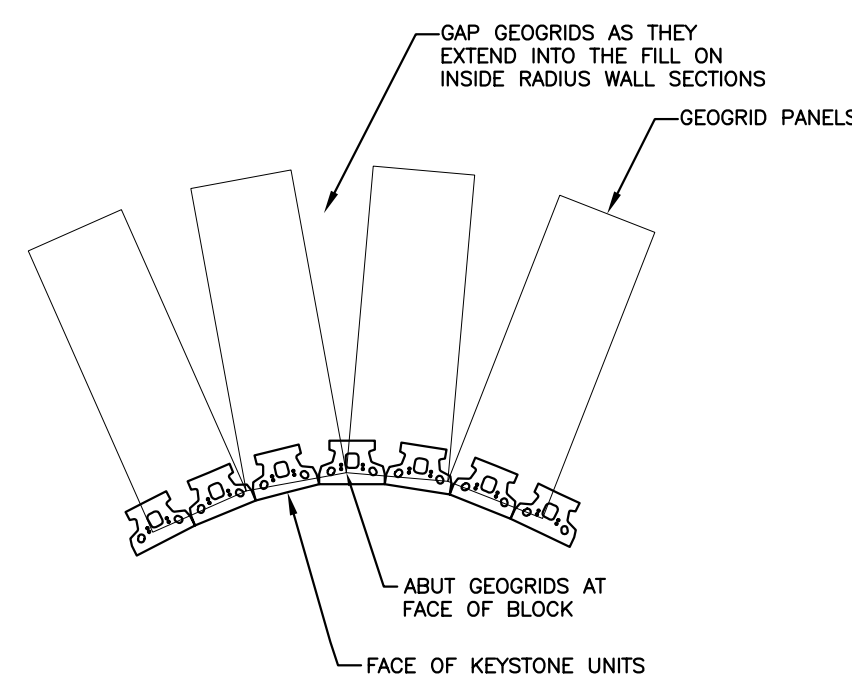
RADIUS WALL DETAIL NOT TO SCALE
