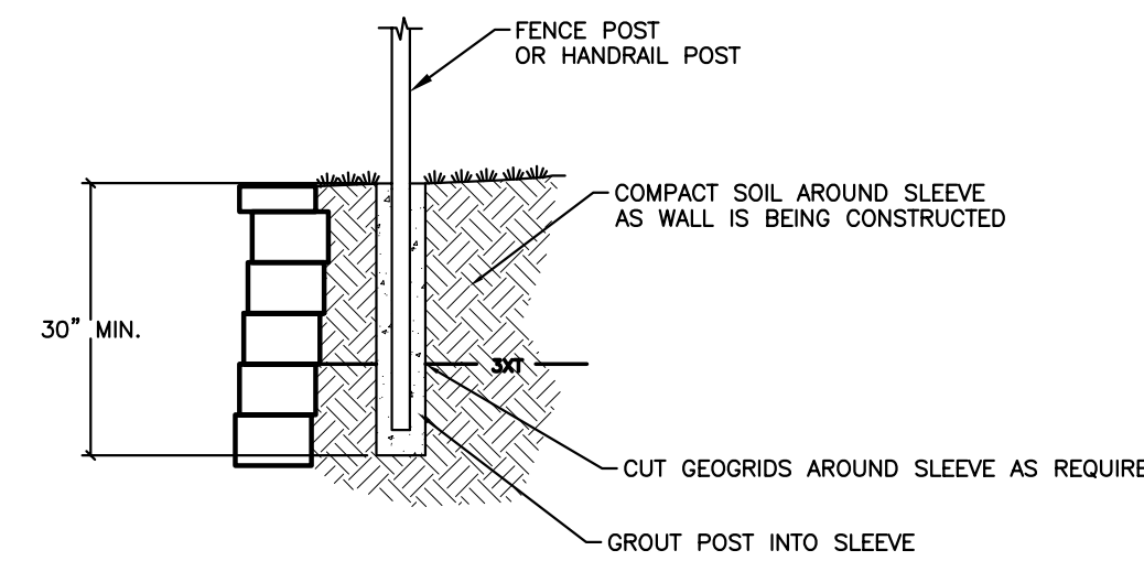
FENCE DETAIL NOT TO SCALE
