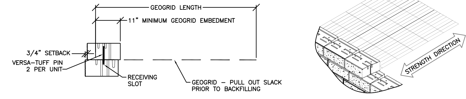
CONNECTION DETAIL NOT TO SCALE
