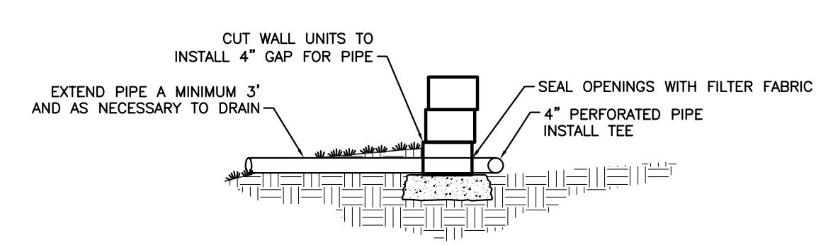
PERFORATED PIPE OUTLET NOT TO SCALE
